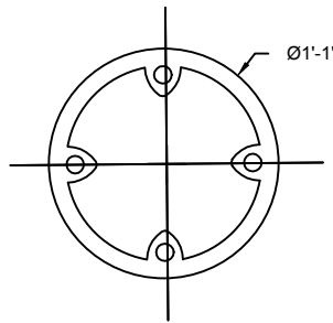
13" 4 HOLE ANCHOR BOLT CIRCLE STANDARD
