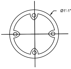
13" 4 HOLE ANCHOR BOLT CIRCLE STANDARD
