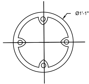
13" 4 HOLE ANCHOR BOLT CIRCLE STANDARD
