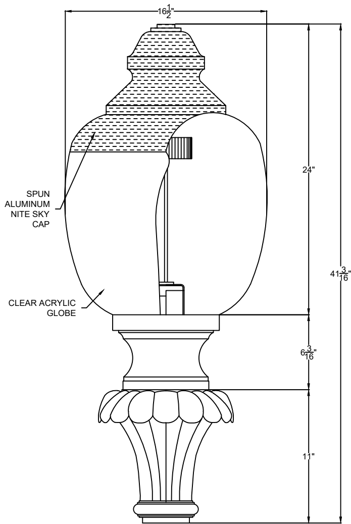
SIDE VIEW SCALE: 1 1/2" = 1'-0" 1
