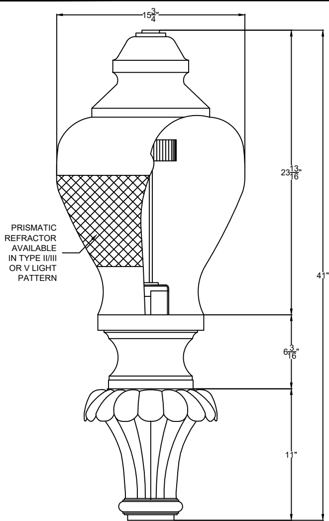
SIDE VIEW 1 SCALE: 1 1/2" = 1'-0"
