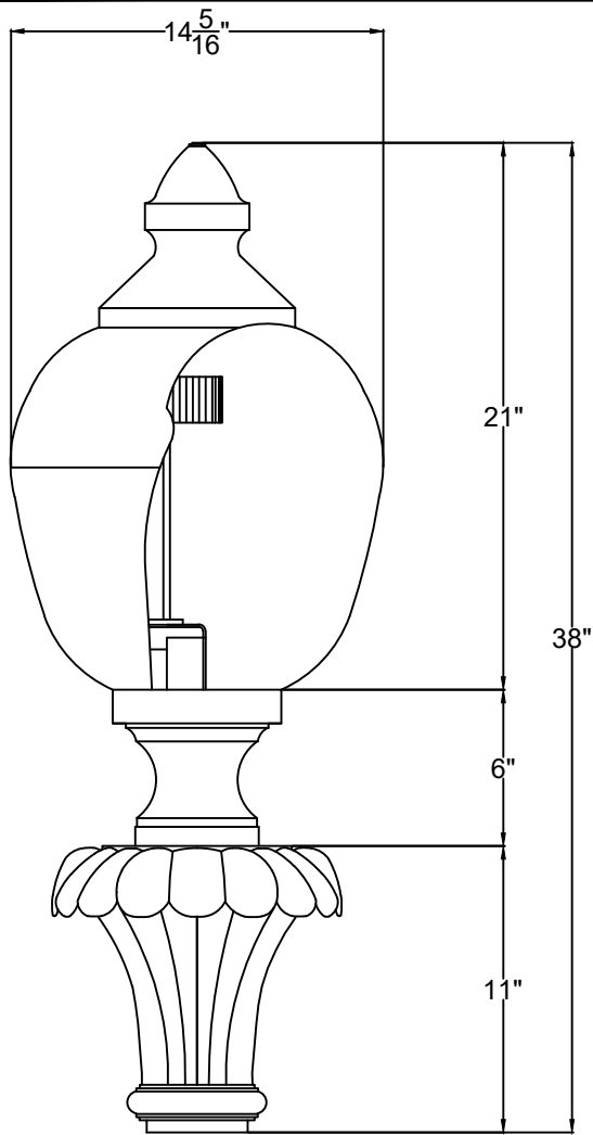
SIDE VIEW 1 SCALE: 1 1/2" = 1'-0"
