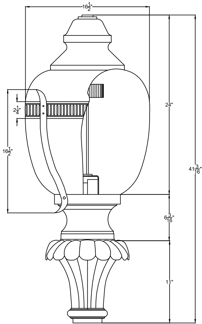
SIDE VIEW 1 SCALE: 1 1/2" = 1'-0"
