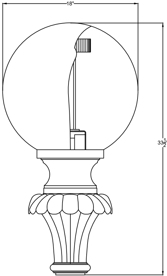
SIDE VIEW SCALE: 1 1/2" = 1'-0" 1
