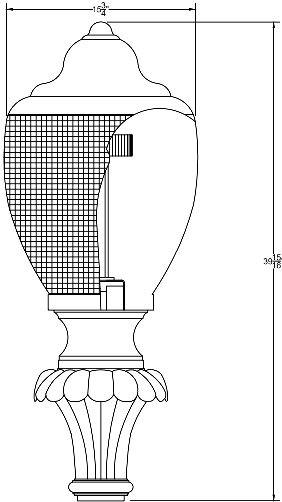
SIDE VIEW 1 SCALE: 1 1/2" = 1'-0"
