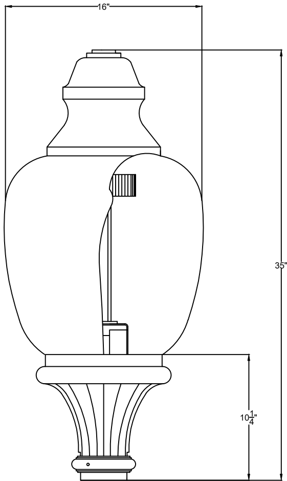
SIDE VIEW 1 SCALE: 1 1/2" = 1'-0"
