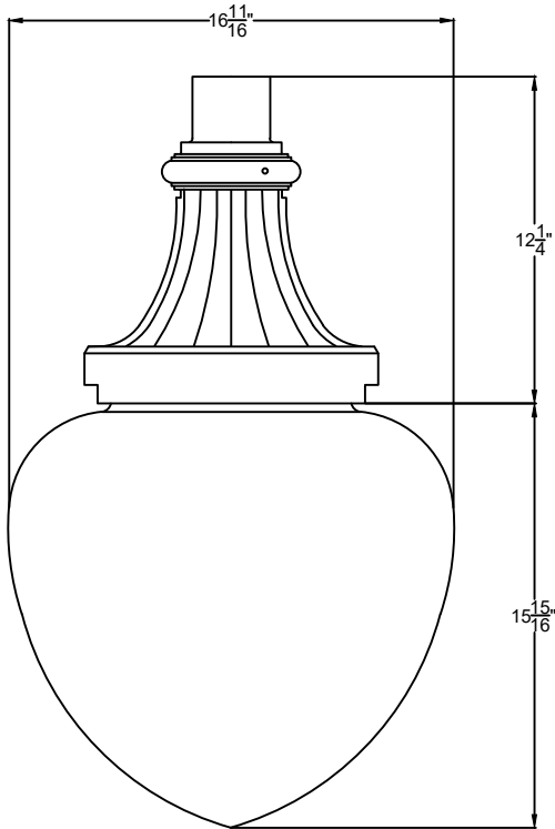
SIDE VIEW SCALE: 1 1/2" = 1'-0" 1
