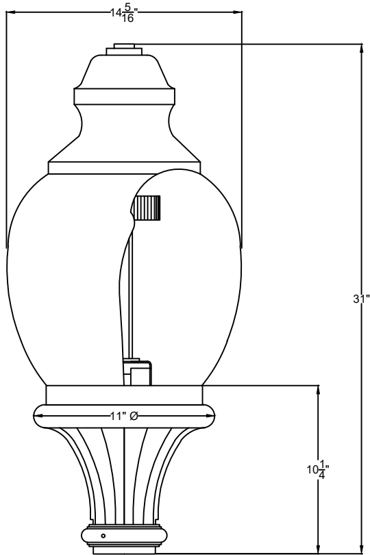
SIDE VIEW 1 SCALE: 1 1/2" = 1'-0"
