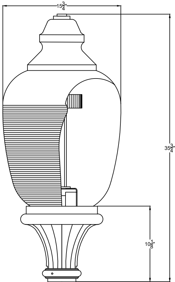
SIDE VIEW 1 SCALE: 1 1/2" = 1'-0"
