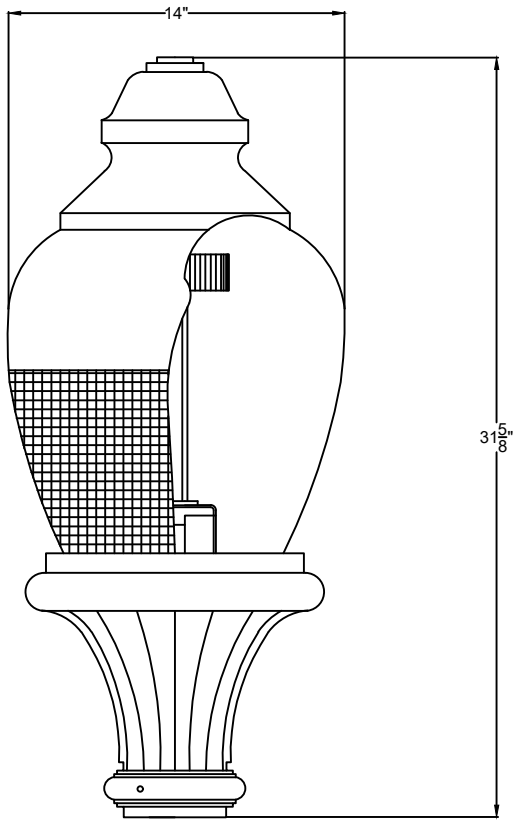
SIDE VIEW 1 SCALE: 1 1/2" = 1'-0"
