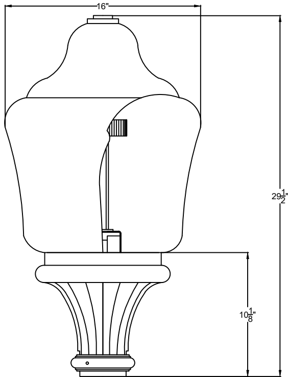
SIDE VIEW SCALE: 1 1/2" = 1'-0" 1
