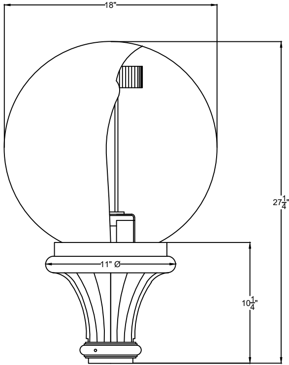
SIDE VIEW SCALE: 1 1/2" = 1'-0" 1
