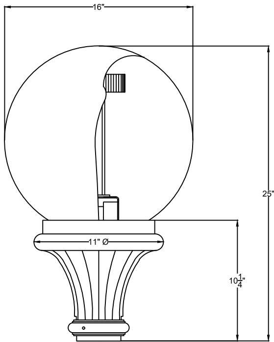
SIDE VIEW 1 SCALE: 1 1/2" = 1'-0"
