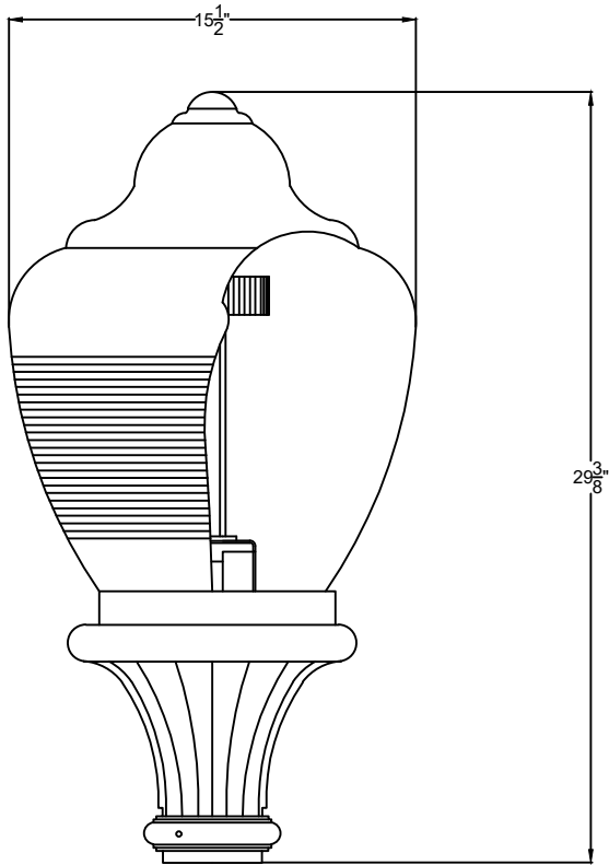
SIDE VIEW 1 SCALE: 1 1/2" = 1'-0"
