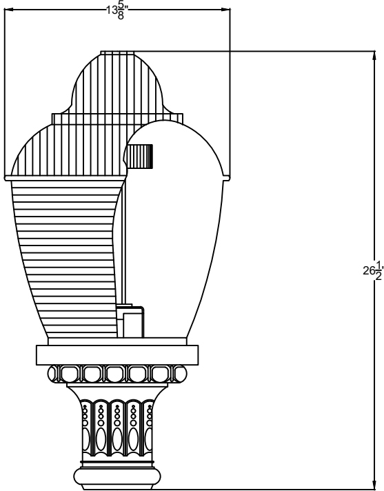
SIDE VIEW 1 SCALE: 1 1/2" = 1'-0"
