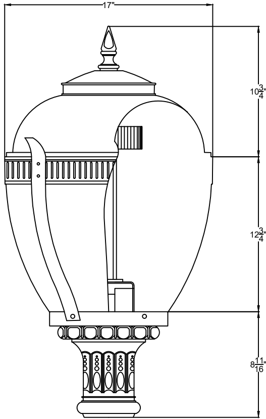
SIDE VIEW 1 SCALE: 1 1/2" = 1'-0"
