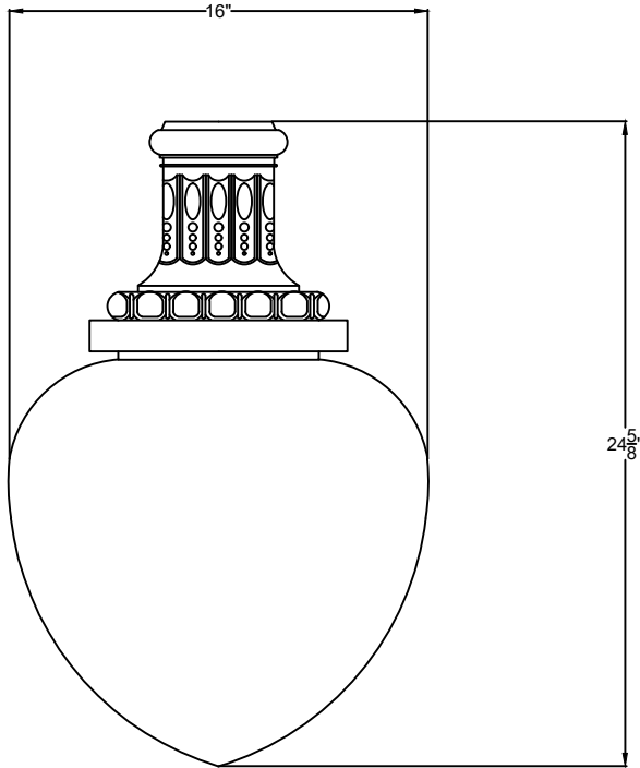
SIDE VIEW SCALE: 1 1/2" = 1'-0" 1
