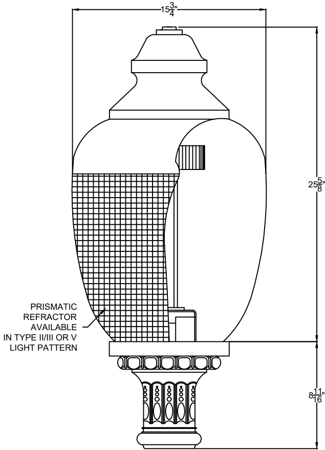
SIDE VIEW 1 SCALE: 1 1/2" = 1'-0"
