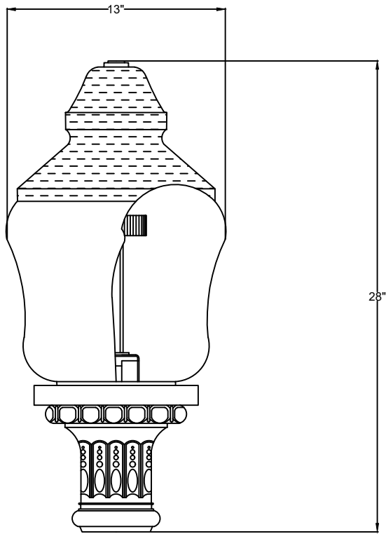
SIDE VIEW 1 SCALE: 1 1/2" = 1'-0"
