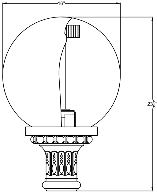
SIDE VIEW 1 SCALE: 1 1/2" = 1'-0"
