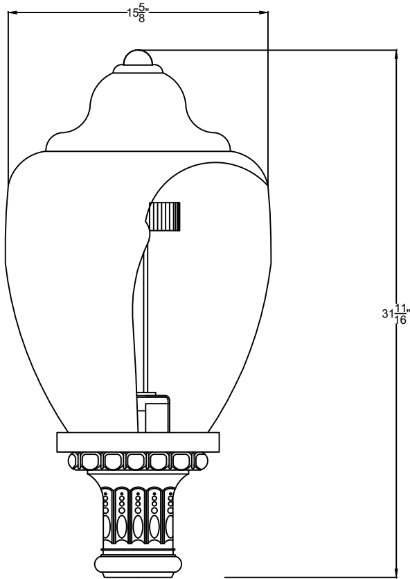
SIDE VIEW 1 SCALE: 1 1/2" = 1'-0"
