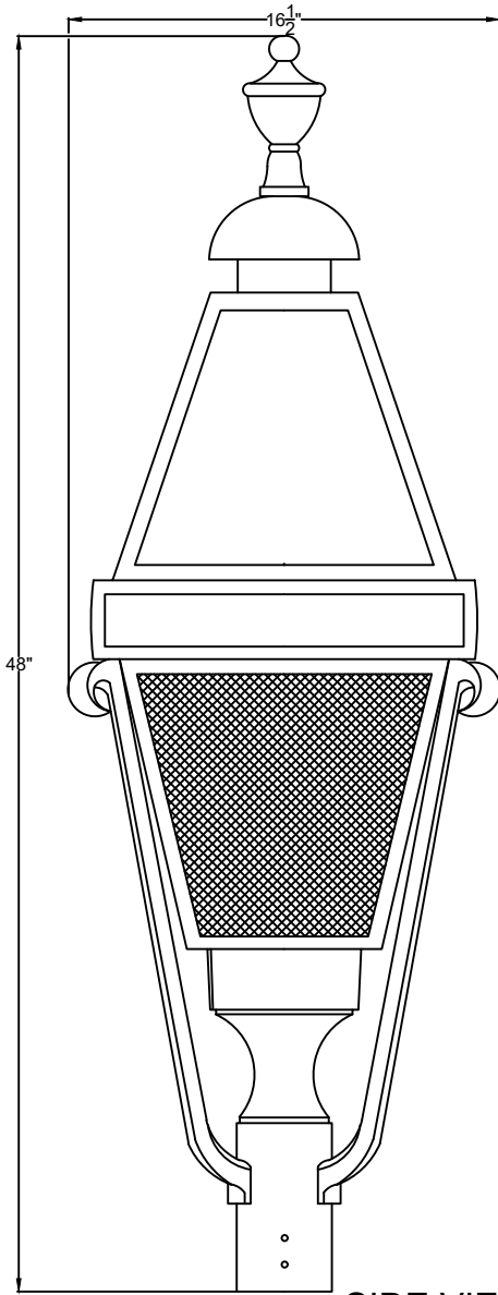
SIDE VIEW SCALE: 1 1/2" = 1'-0" 1
