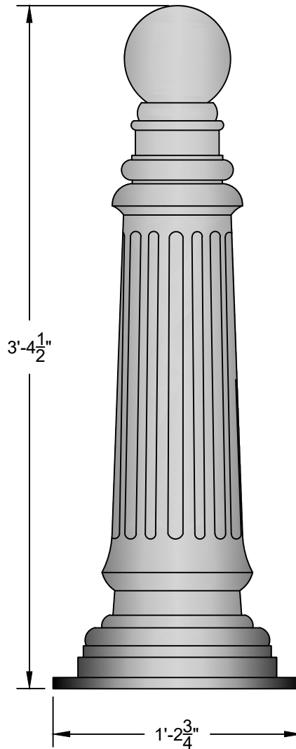
SIDE VIEW SCALE: 1 1/2" = 1'-0" 1
