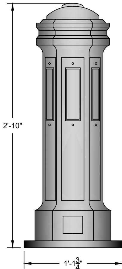
SIDE VIEW 1 SCALE: 1 1/2" = 1'-0"
